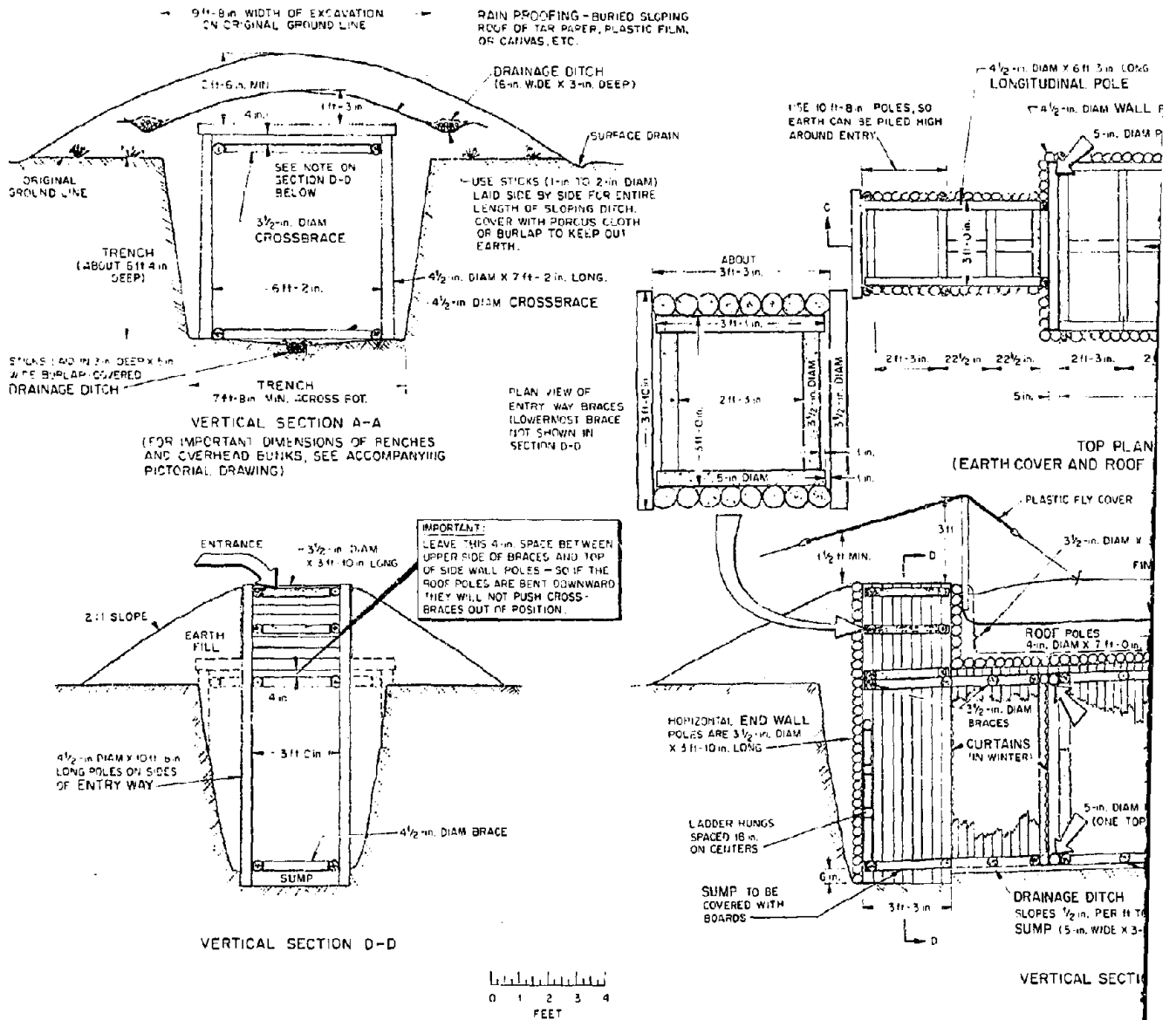
Fig. A-1.2. Small-Pole Shelter, Plan and Elevation
